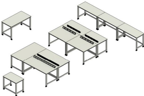
3D drawing of mobile laboratory table layout
